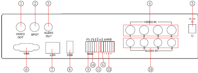
Fig 2.1 Rear view for 4-ch DVR
